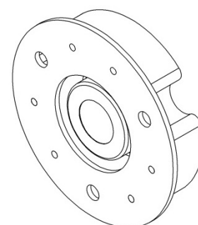
FIGURE 1.5 NV K135 COUPLING (ENGINE SIDE)
